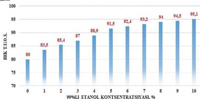
3–rasm. Etil spirtini AI-80 avtomobil benzinining detonatsion barqarorligiga ta'siri
