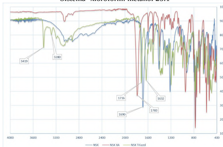
1-rasm. Naftil sirka kislotasining 3-amino 1,2,4-triazol bilan olingan amidining IQ spektrlari
