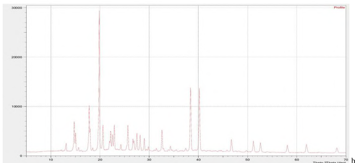
Fig. 1. Röntgenographs: a- \text{CH}_3\text{CONH}_2 , b- \text{Ba}(\text{NO}_3)_2 \cdot 2\text{CH}_3\text{CONH}_2
