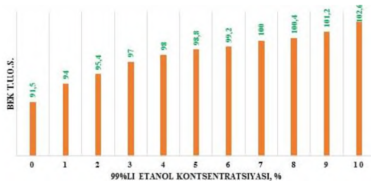
4-rasm. Etil spirtini AI-92 avtomobil benzinining detonatsion barqarorligiga ta'siri
