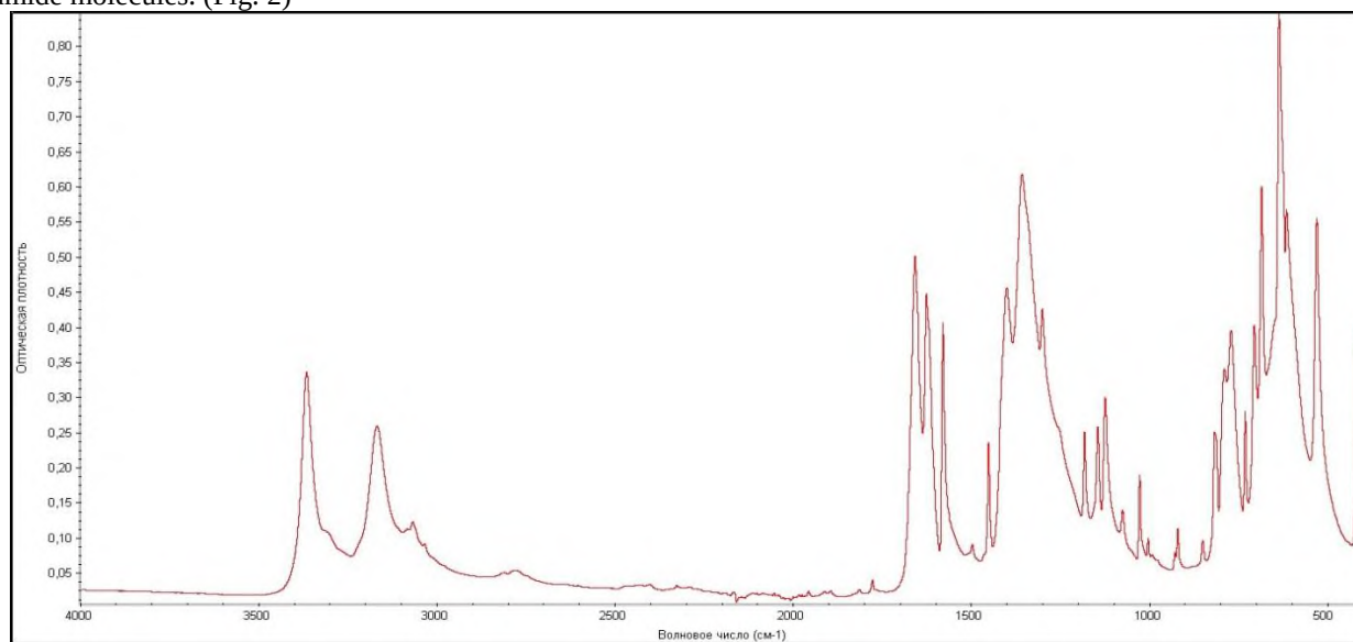
Fig. 2. IR absorption spectrum of the complex compound of barium nitrate with acetamide – \text{Ba}(\text{NO}_3)_2 \cdot 2\text{AA} .
