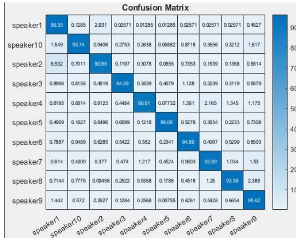
2 -rasm. Adaptivfiltrningqo'llanilishi
