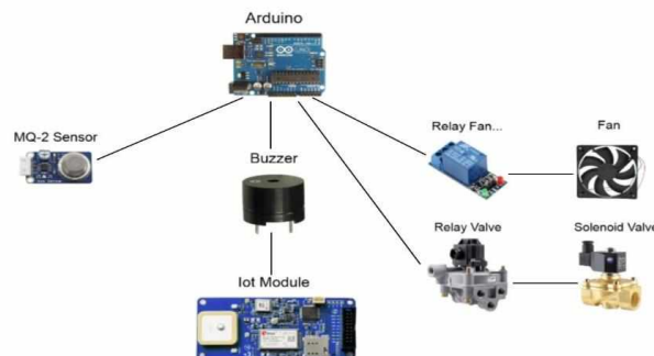
Figure 1. Smart air extractor system diagram
