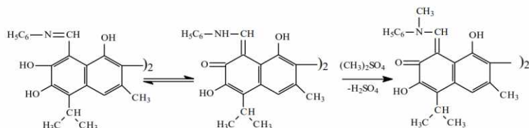
4-rasm: Dianilingossipolning metillanishi
