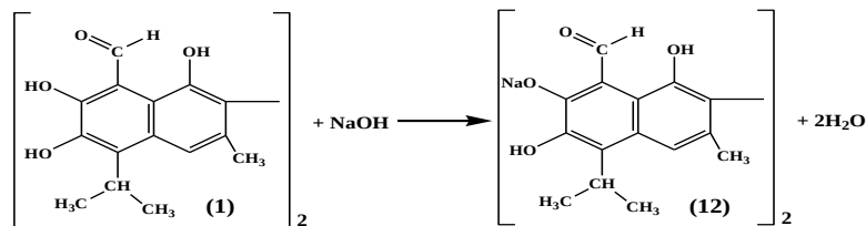
7-rasm: Gossipolat tuzlar hosil bo'lishi
