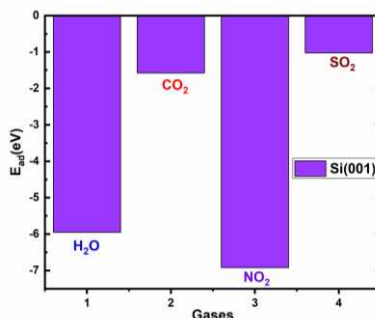
Rasm3. Gaz molekularining Si(001) yuzasida adsorbsion energiyalari.
