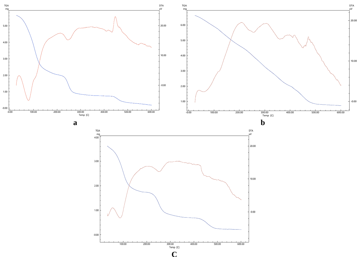
Figure 1. TGA curves for PVC sorbents modified with DEA, MEA, and DEDC
